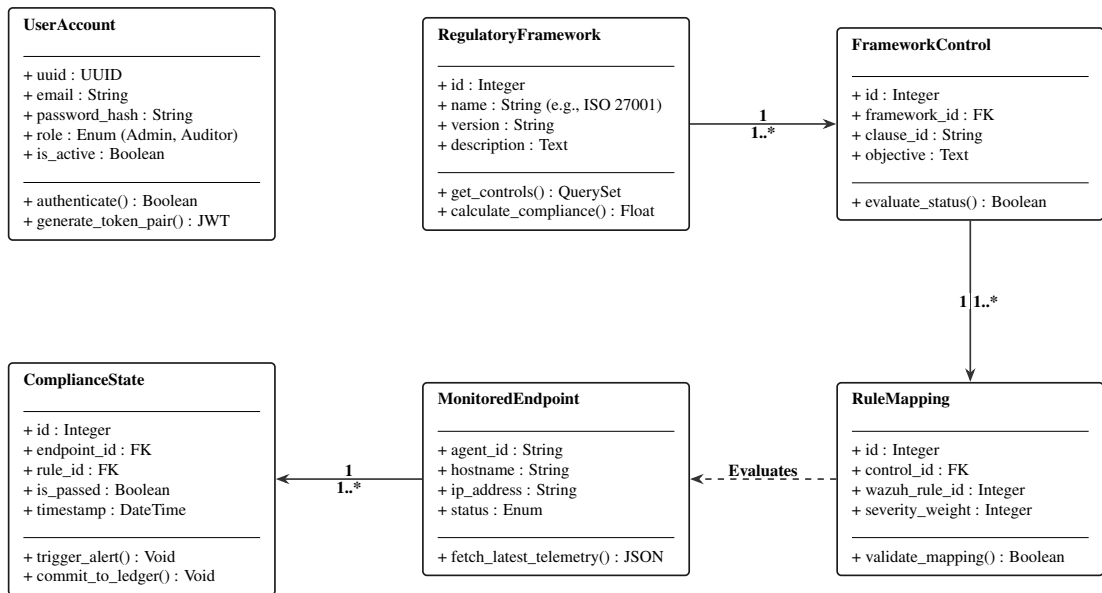
Figure 4.18: UML Class Diagram: Core Object-Relational Models
